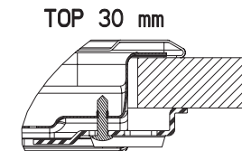
TOP 30 mm
